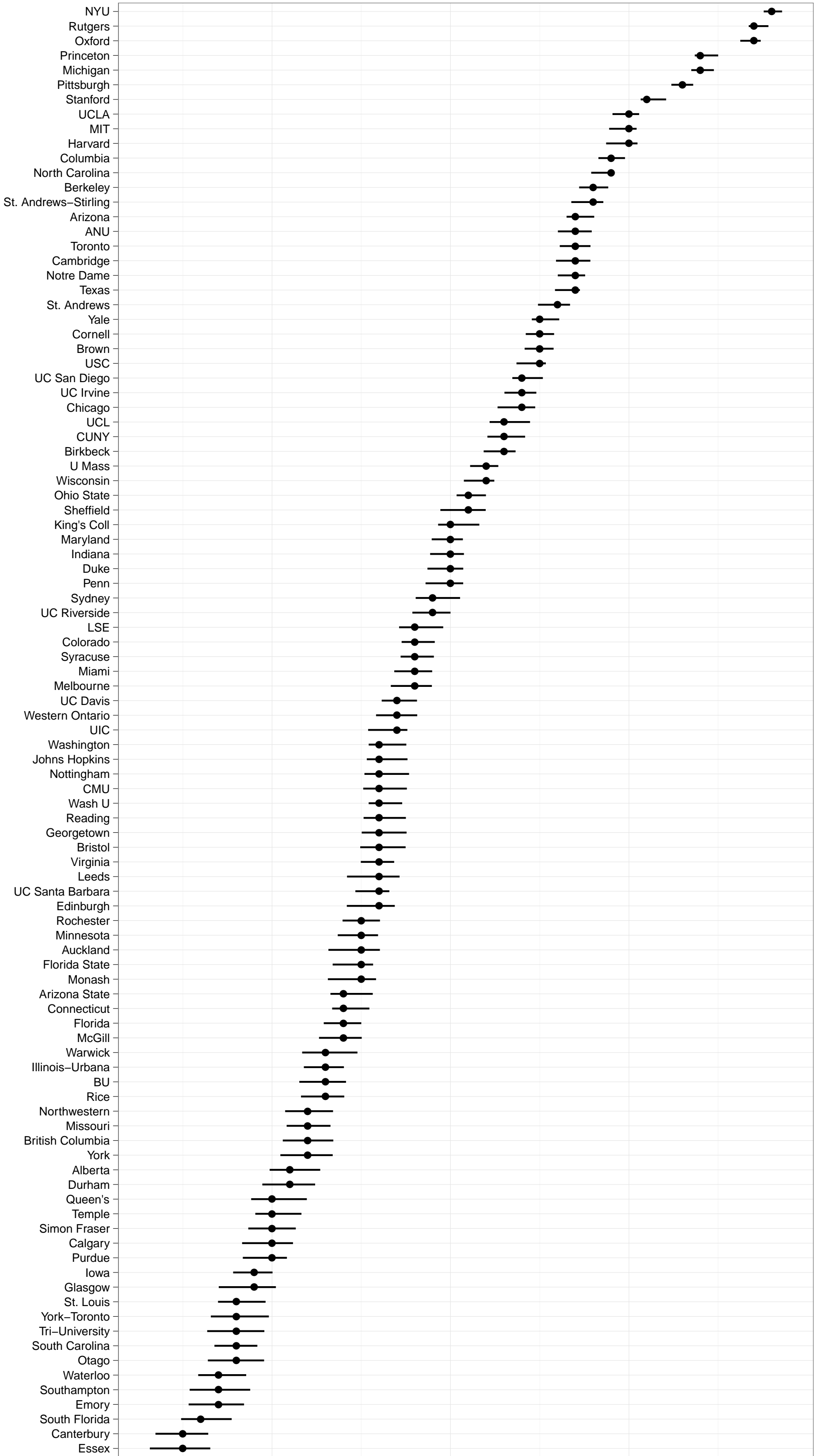
2006 PGR Scores with bootstrapped 95% Confidence Intervals
