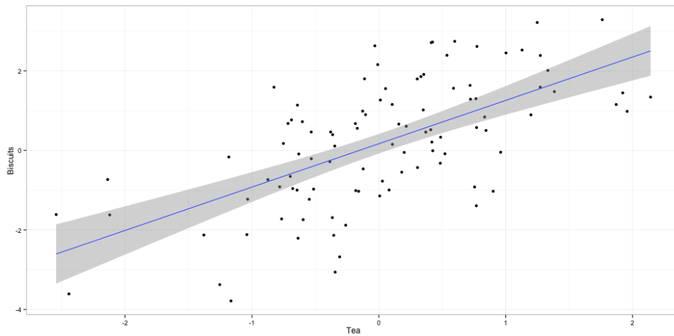
Figure 1: Tea and Biscuits are correlated but there may be identifiability issues.
